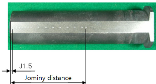
[Fig. 4] (a) Cooling apparatus for Jominy test (b) Jominy hardness test site (test position : 1.5, 3, 5, 7, 9, 11, 13, 15, 20, 25, 30 mm)
