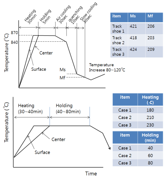
[Fig. 6] Heat cycle of (a) quenching and (b) tempering
