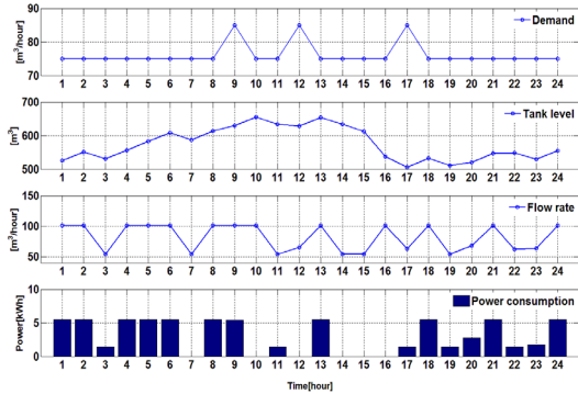
[Fig. 10] PSO control with variable power(variable demand)
