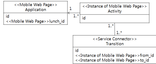
Fig. 3. MetaModel for Dynamic Mobile Web Service
