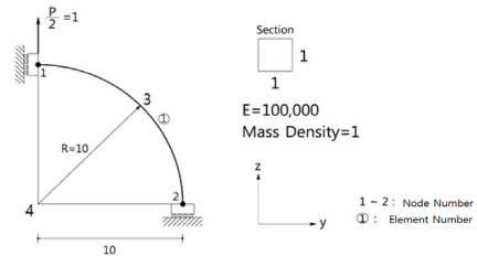
Fig. 6. Example of Analysis Model
