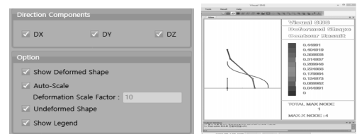
Fig. 14. Displacement contour of the curved beam
