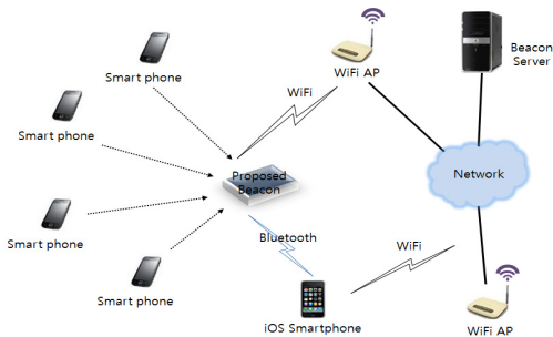
Fig. 1. System Configuration
