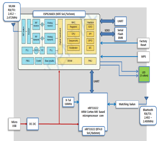
Fig. 2. Block Diagram
