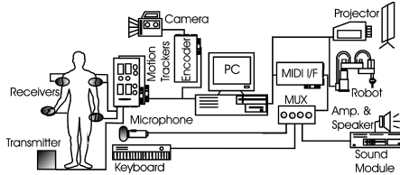
Fig. 1. An intention capture and mapping system
