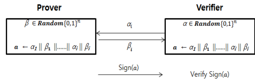
Fig. 1. Distance-Bounding Protocol
