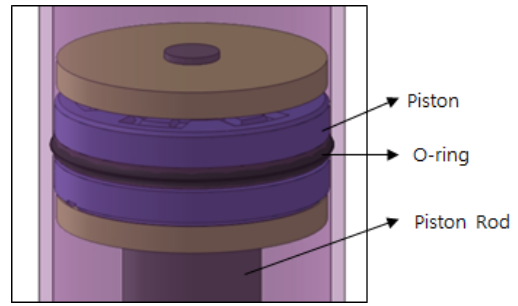
Fig. 5. Piston location at compression
