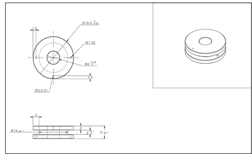
(a) Pipe type orifice
