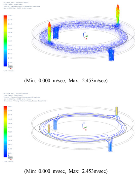
Fig. 13. Velocity distribution at two orifice
