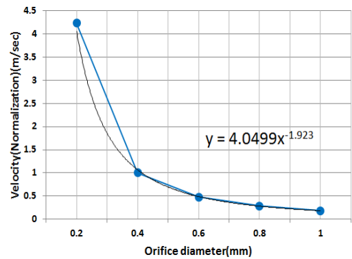
(b) Velocity according to orifice diameter and curve fitting of data
