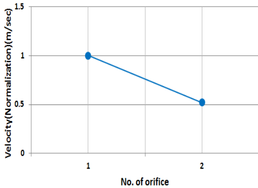
Fig. 14. Velocity according to No. of orifice
