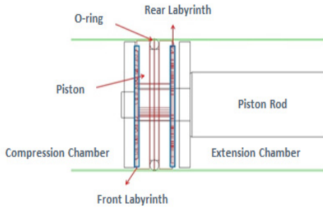
Fig. 2. Schematic diagram of piston package
