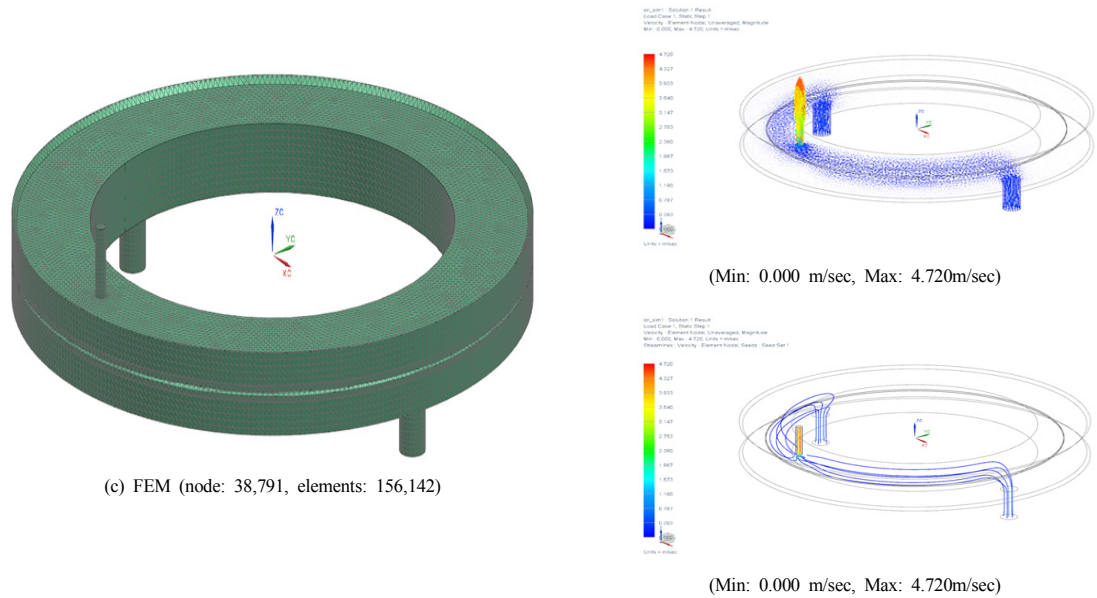
Fig. 11. Velocity distribution of pipe type orifice
