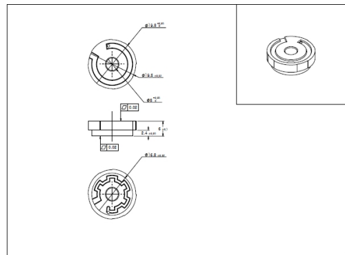
(b) Labyrinth type orifice
