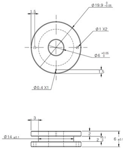
(a) 2d CAD of pipe type orifice
