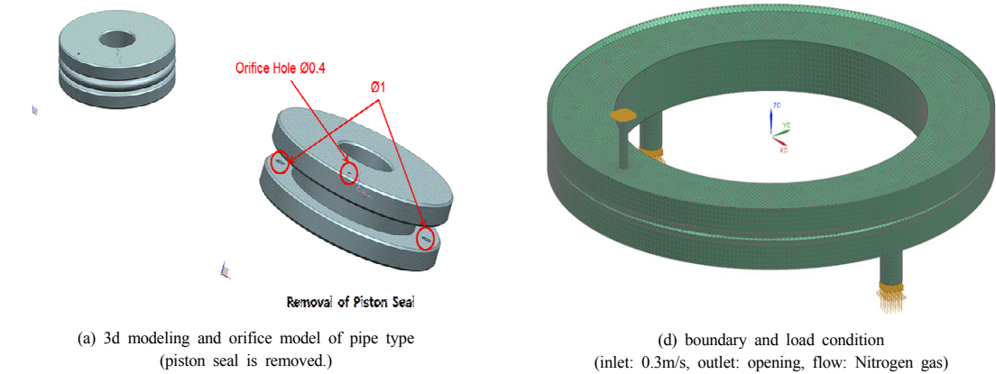
Fig. 10. Simulation preparation of pipe type orifice
