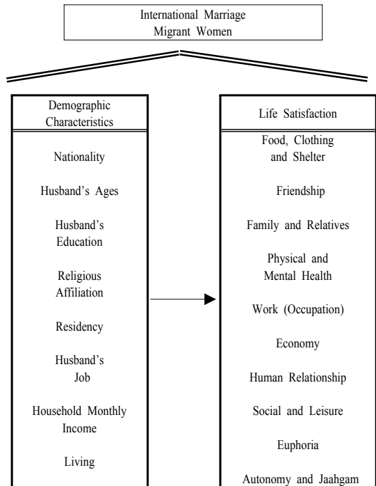
Fig. 1. Research model
