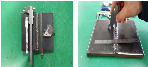
[Fig. 7] Visual inspection of the equipment and experimental
