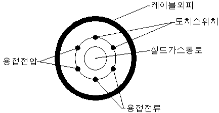
[Fig. 5] Section of remote control torch welding cable
