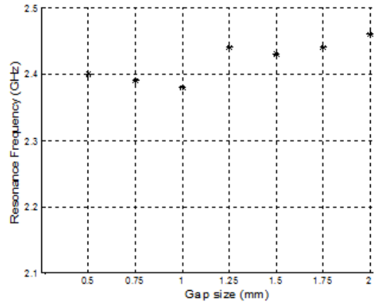
Fig. 4. Antenna resonance frequency versus gap size
