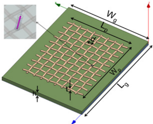
Fig. 1. Simulation model of conductive fiber antenna
