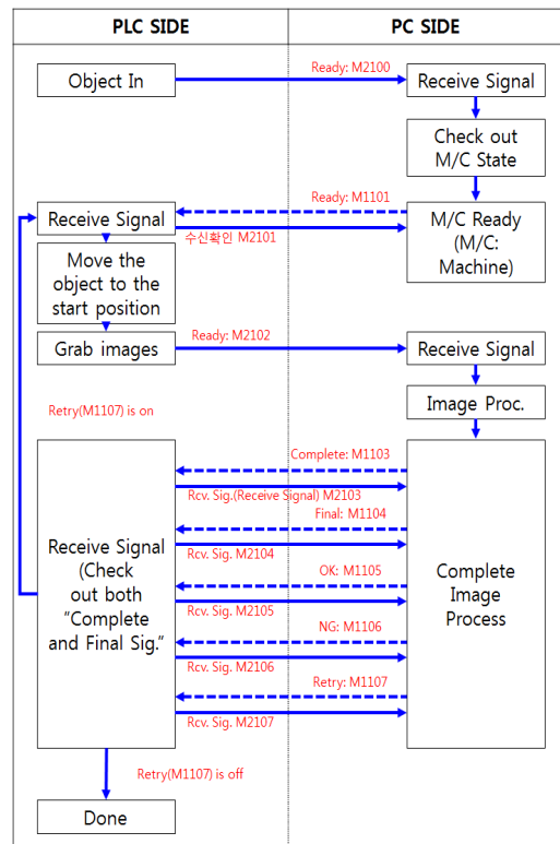
Fig. 3. PC/PLC interface
