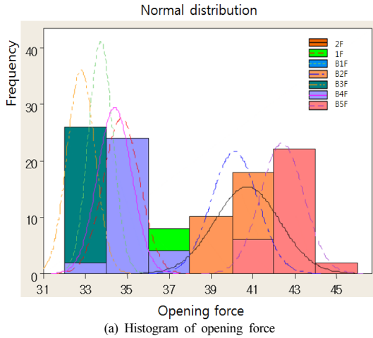
Fig. 5. Distribution chart for opening force measuring values after a smoke control system operates.
