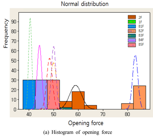
Fig. 6. Histogram and probability of opening force measurement values before a smoke control system operates (Access door closed completely)
