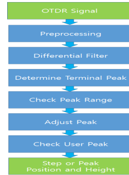
Fig. 3. Block Diagram of OTDR signal analysis
