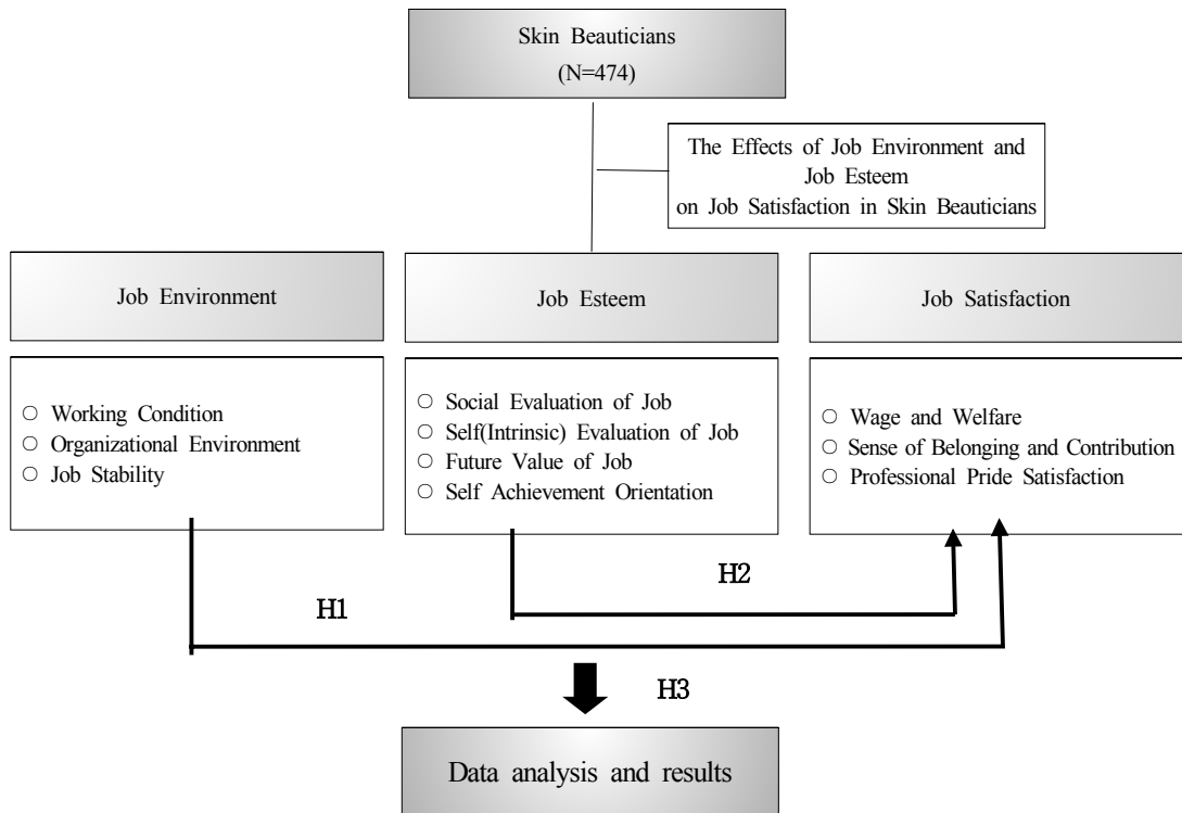
Fig. 1. Research Model
