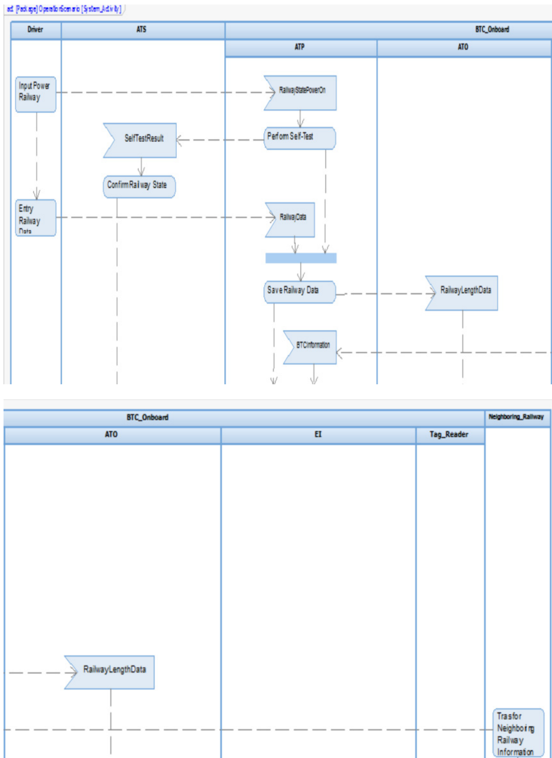
Fig. 4. Activity Diagram of Train-centric Train Control System
