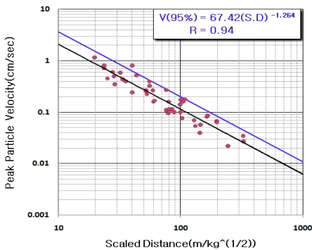
Fig. 1. Relation of Peak Particle Velocity to Square root Scaled Distance
