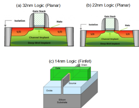
Fig. 5. Transistor architecture comparison (Source : ITRS, Wikipedia)
