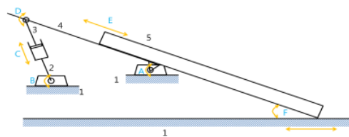
Fig. 2. Geometric diagram of sliding deck system
