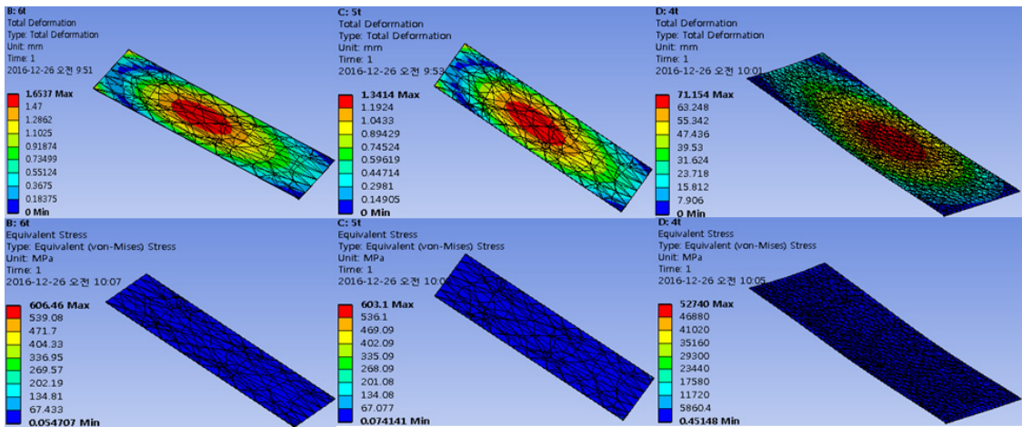
Fig. 7. Analysis result of ATOS80 (deformation, equivalent stress) (a)In case of 6mm (b)In case of 5mm (c)In case of 4mm
