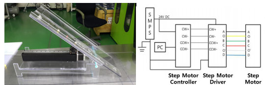
Fig. 4. Down scale model and circuit diagram
