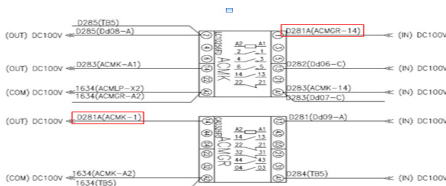
Fig 7. Wiring Analysis of the GDB in TC car
