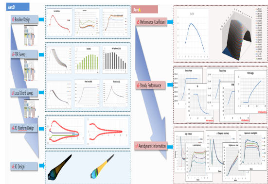
Fig. 6. AeroD module(left), AeroA module(right)
