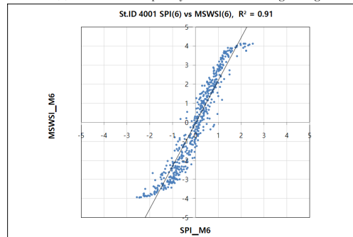
(c) SPI vs MSWSI plot by six month moving average
