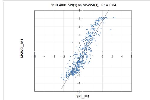
(a) SPI vs MSWSI plot by one month
