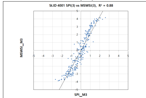
(b) SPI vs MSWSI plot by three month moving average
