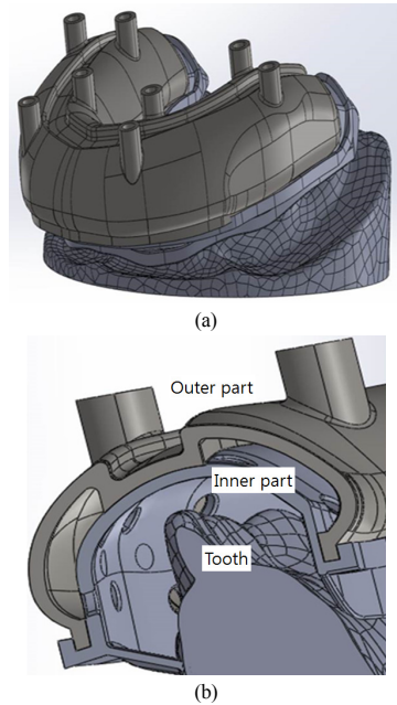
Fig. 6. Assemble model of vacuum oral cleaner and teeth: (a) assemble model; (b) sectional view
