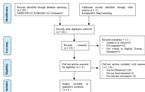
Fig. 1. Flow diagram for study selection
