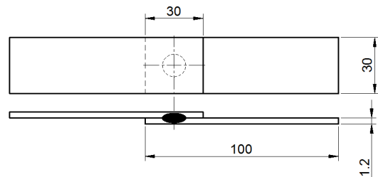
Fig. 1. Schematic drawing of the specimen (Unit: mm)
