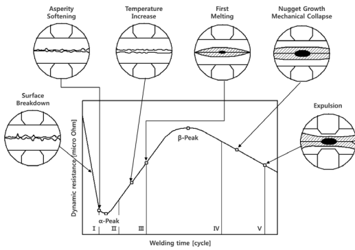
Fig. 4. Typical dynamic resistance curve
