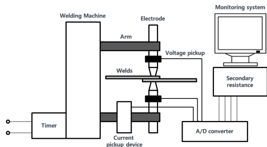
Fig. 3. Schematic diagram of the conventional secondary dynamic resistance monitoring system
