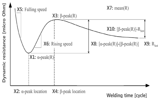
Fig. 5. Secondary dynamic resistance pattern and feature extraction
