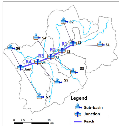
Fig. 2. Model implementation generated by HEC-HMS
