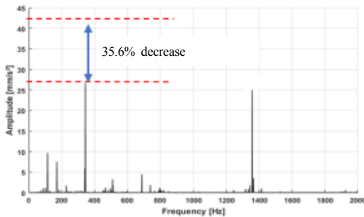
Fig. 13. Frequency response of cabin frame with optimized anti-vibration rubber assembly
