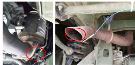
Fig. 4. Exhaust gas temp. measurements on various operation environments
