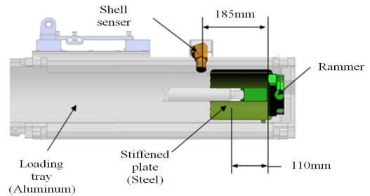
Fig. 1. Internal structure of the flick rammer on self propelled artillery
