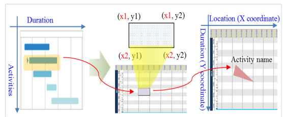
Fig. 6. Coordinate system for conversion of Gantt chart to linear schedule chart
