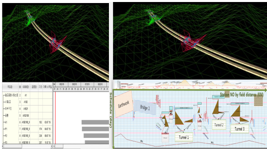
Fig. 8. Simulation function in current 4D and linear 4D CAD systems
