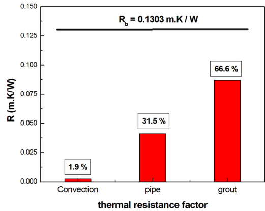
Fig. 5. Contribution of individual thermal resistance
