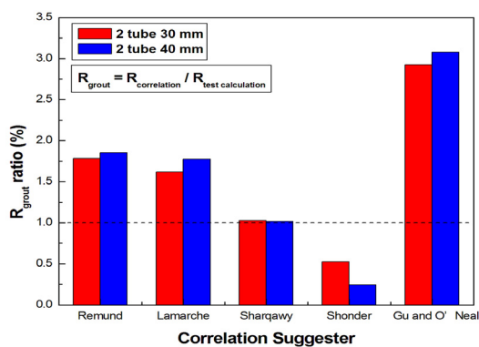
Fig. 7. Variation of the grout thermal resistance with correlation equation and pipe diameter.
