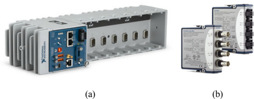
Fig. 5. Data aquisition system(NI) (a) Controller chassis (b) Voltage measuring module
