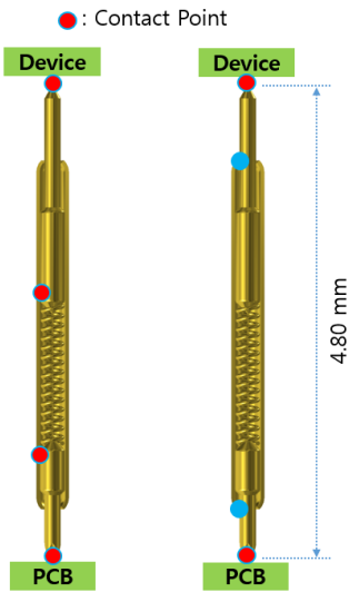
(a) Plunger inner contact (b) Barrel inlet contact
