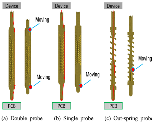
Fig. 5. Components of the double, single and out-spring probes
