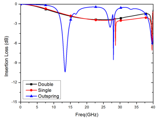
Fig. 7. Insertion loss of double, single and out-spring probes
