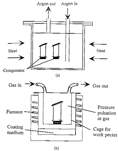
Figure 1. Pack cementation processes: (a) Without pressure(Ar gas), (b) With pressure(Air).
