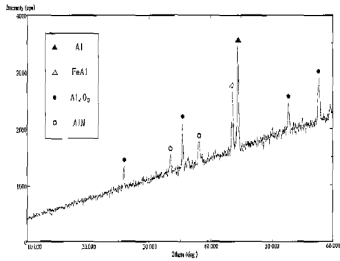
Figure 3. XRD pattern of coating powder after calorizing at air condition.
