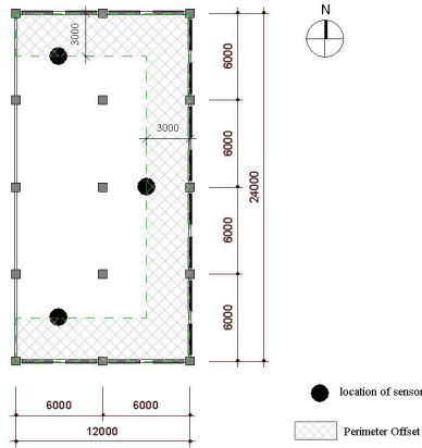
Fig. 2. Plan of Test Building
