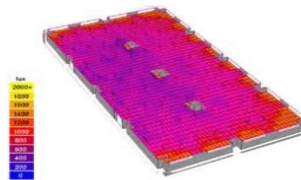
Fig. 7. Lighting Analysis of Daylight
