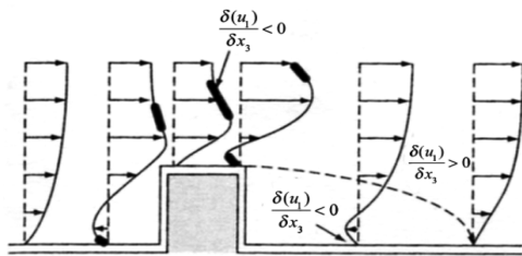
(a) Distribution of Main Shear Layer ( \sigma U_1/\sigma x_3 )
