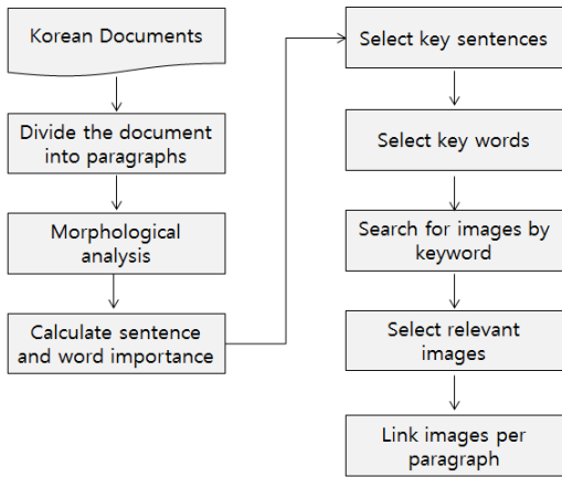
Fig. 1. Overall Process for Image Retrieval System
