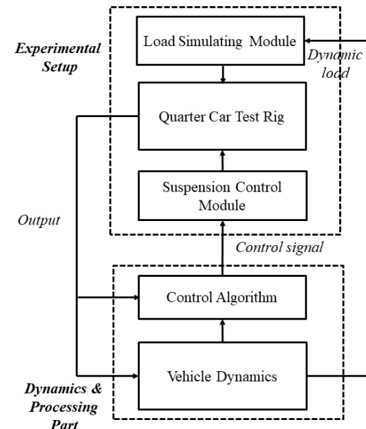
Fig. 3. Configuration of overall lateral motion control system
