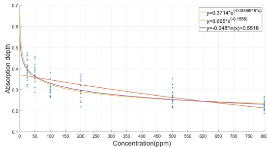
Fig. 3. \text{NO}_2 concentration versus absorption depth with three concentration estimation equations
