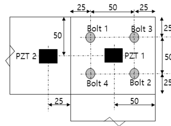
Fig. 1. Shape of the specimen (lengths in mm).
