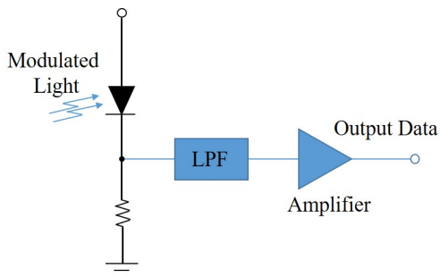
Fig. 1. A block diagram of optical receive system
