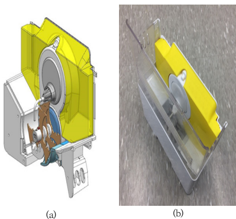
Fig. 6. Modified ice dispenser (a) Model of modified ice dispenser (b) Assembly of modified ice dispenser
