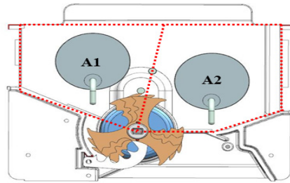
Fig. 10. Locations of the two ice breakers
