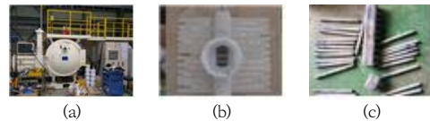
Fig. 1. (a) High frequency induction furnace, (b) Lost wax mold, (c) Casting specimens.
