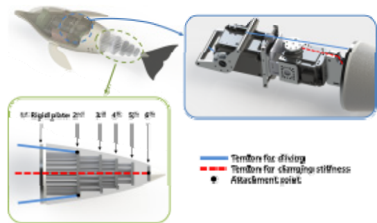
Fig. 7. Schematic design of the robotic dolphin driving system. Adapted and modified from [20]
