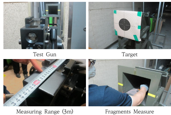
Fig. 6. Test procedure
