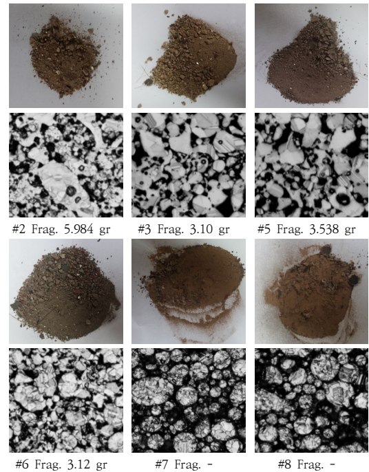
Fig. 9. Microscope and fragments photographs of samples
