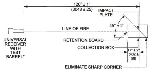
Frangible ammunition test equipment
