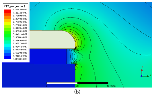
Fig. 4. Comparing of electric field distribution with difference of static ring's curvature (a) Electric field distribution with adopted 1mm radius of curvature static ring (b) Electric field distribution with adopted 10mm radius of curvature static ring
