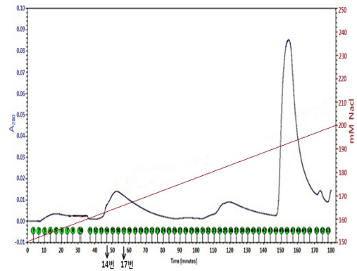
Fig. 7. DEAE Sepharose CL-6B chromatogram of fractions including soluble rhEGF resulted from first IEX (Ion Exchange chromatography).
