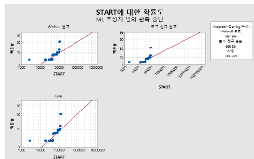
Fig. 7. Distribution Analysis
