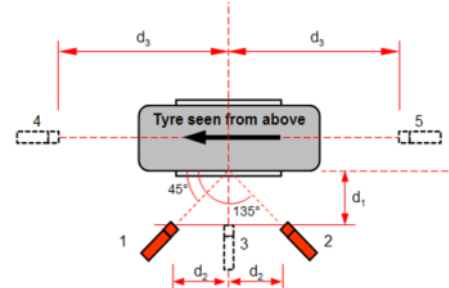
(b) Microphone position when the tire is viewed from above
