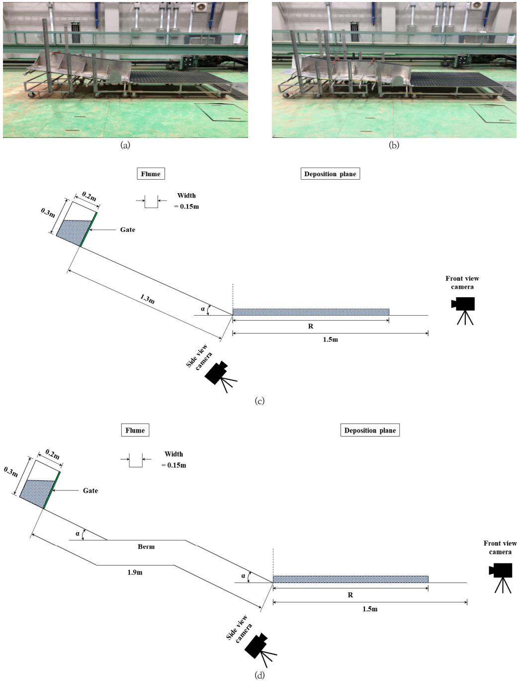
Fig. 1. Experimental setups for laboratory tests. (a) Image of the linear channel test, (b) Image of the one-stepped channel test, (c) Schematic diagram of the linear channel test, (d) Schematic diagram of the one-stepped channel test
